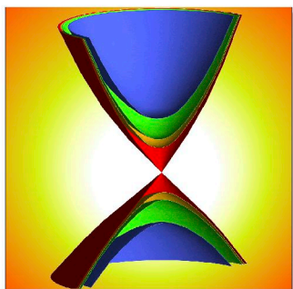
Unexpected mass acquisition of Dirac fermions in TlBi(S_{1-x}Br_x)_2
