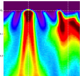
Band dispersion of LiFeO_3
