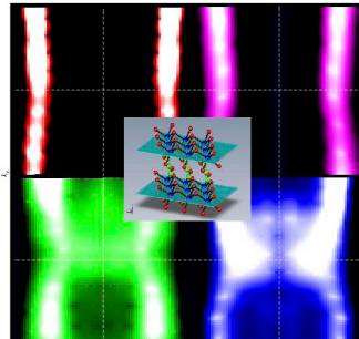
Doping evolution of 3D Fermi surface in NaCo_2O_7
