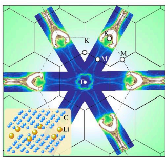
Fermi surface of Li-intercalated bilayer graphene
