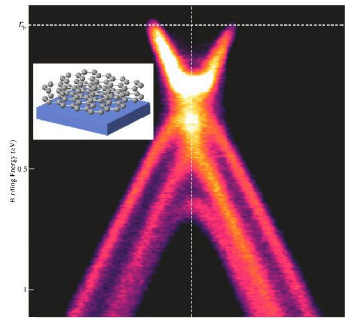
Band dispersion of multilayer graphene
