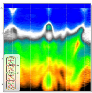
Valence-band structure of TiBiSe_2
