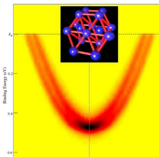
Spin split surface states of Au(111)
