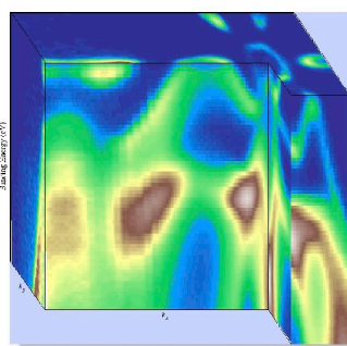
Band dispersion and Fermi surface of Bi(111)
