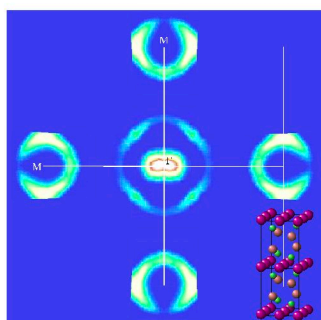
Fermi surface of LiFeO_3
