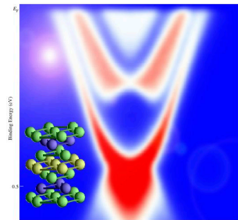
Band dispersion of topological insulator PbBi_2Te_4
